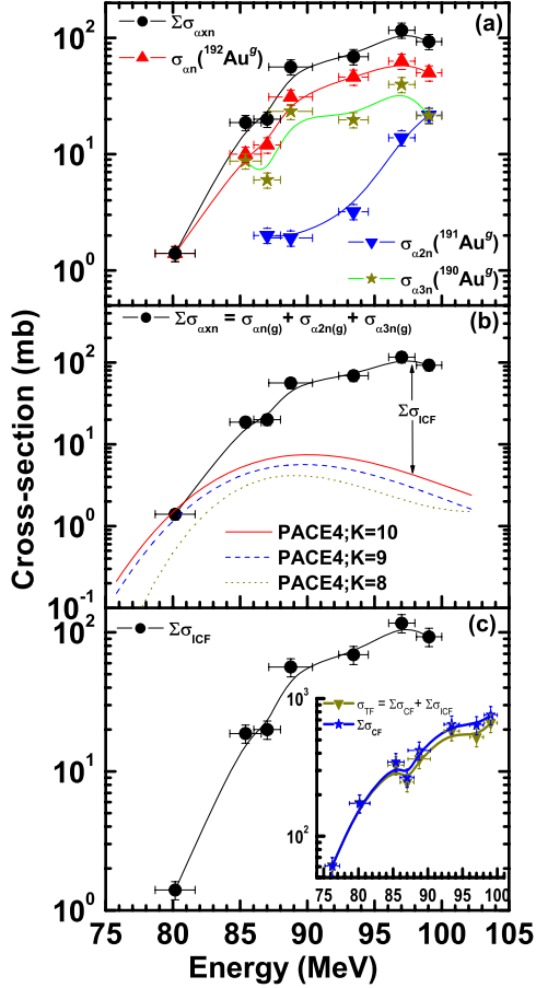
FIG. 1: Measured EFs for (a) \alpha xn ( x = 1, 2 & 3 ) channels, (b) sum of the \alpha xn channels; measured as well as calculated using PACE4 (c) sum of \sigma_{ICF} ( \Sigma\sigma_{\alpha xn} ) channels. Inset shows cross-sections for the sum of both CF and ICF channels, and CF channels separately.
