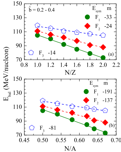
FIG. 1: E_{bal} as a function of N/Z (upper panel) and N/A (lower panel) of system. Various lines and symbols are explained in the text.
