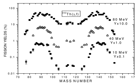
Fig. 1. Yield distribution in ^{232}\text{Th}(\gamma, f) at end point Bremsstrahlung energy of 10, 40 and 80 MeV.
