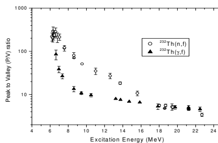
Fig.2. Plot of P/V in ^{232}\text{Th}(\gamma, f) and ^{232}\text{Th}(n, f) .
