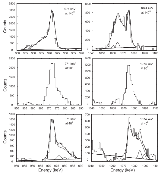
FIG. 1: The obtained lineshape for the transition of energy 971 keV and 1074 keV in the negative parity band of ^{101}\text{Pd} [8] at 40^\circ , 90^\circ , and 140^\circ angles.
