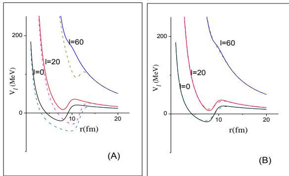
Fig. 1(Color online) (A) Variation in total potential for {}^6\text{He}+{}^{209}\text{Bi} system with radius parameter 1.17 fm (solid line) and 1.5 fm (dashed line) for different l values with a=0.5\text{fm} . (B) Same as in (A) but with diffuseness 0.5fm (solid line) and 0.7 fm (dashed line) for different l values with r_0 fixed at 1.17fm.
