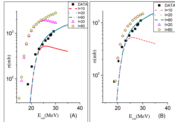
Fig. 2(Color online) (A) Fusion excitation functions of {}^6\text{He}+{}^{209}\text{Bi} system at around barrier energies corresponding to r_0=1.17 fm (lines) and 1.5 fm (symbols) for different l values with a=0.5\text{fm} . In B same as of (A) but with a=0.5 fm (lines) and 0.7 (symbols) for different l values with r_0 fixed at 1.17fm. The data point in (A) and (B) are taken from ref.[6]
