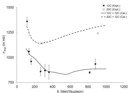
FIG. 2: Energy dependence of the reaction cross sections for ^{12}\text{C} and ^{20}\text{C} on ^{12}\text{C} target.
