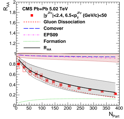
FIG. 1: Calculated nuclear modification factor ( R_{AA} ) of J/\psi as a function of centrality of collisions, compared with CMS measurements [2].
