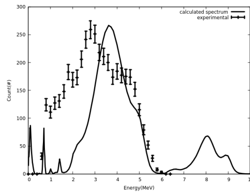
Fig.2 The neutron energy spectrum of Am-Be source measured (preliminary) and simulated [2]
