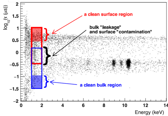
FIG. 2: The \tau distribution at low background configuration for pGe detector [2].
