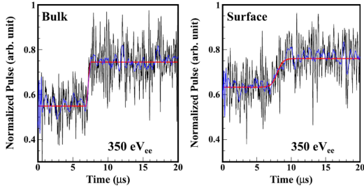
FIG. 1: Typical pulse shape of Bulk (left side) and Surface events (right side) both having 350 eV_{ee} energy are shown along with raw pulses in black, the smoothed (blue) pulses, together with the best-fit functions (red) are also superimposed [2].
