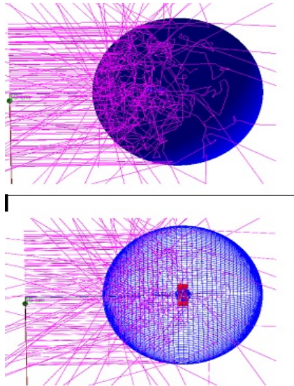
FIG. 1: The scene of neutron irradiation in Geant4, (a) Approximately 10^5 high energy neutrons falling on Bonner Ball, (b) View explaining how neutrons are elastically scattered and few of them are approaching to the crystal which is located in the centre
