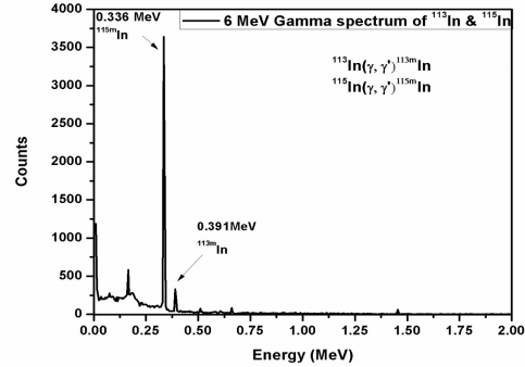
Fig.2: Gamma-ray spectrum of ^{113\text{m}}\text{In} and ^{115\text{m}}\text{In}
