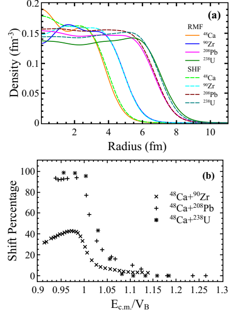
FIG. 1: (a) The RMF (solid lines) and SHF (dashed lines) total radial density distribution for all nucleus involved in considered reactions. (b) Percentage shift vs E_{c.m.}/V_B for ^{48}\text{Ca}+^{90}\text{Zr} , ^{208}\text{Pb} , and ^{238}\text{U} reactions.
