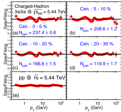
FIG. 2: Ratio of the charged-hadron's yields data and their Modified Tsallis fits as a function of p_T for pp and XeXe collisions at \sqrt{s_{NN}} = 5.44 TeV.
