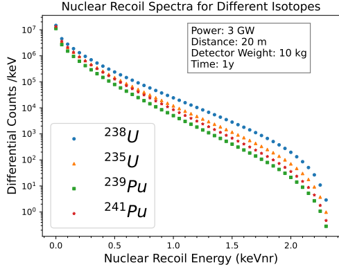
FIG. 1: The nuclear recoil spectrum assuming the entire anti-neutrino flux to be due to a single fissile isotope.
