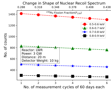
FIG. 3: The different rates of change in CE \nu NS yield with time for different nuclear recoil energy bins.
