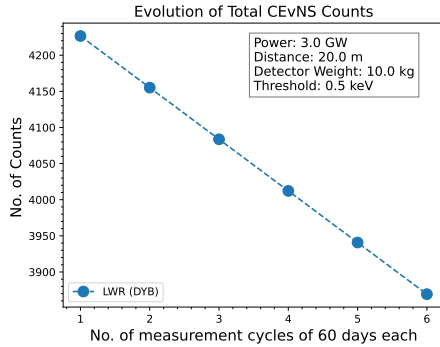
FIG. 2: The evolution of CE \nu NS yield over a fuel cycle for a typical LWR.
