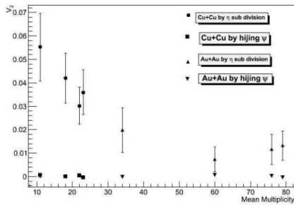
Fig. 1: Elliptic flow variation with mean multiplicity for \pi^- at 200 GeV
