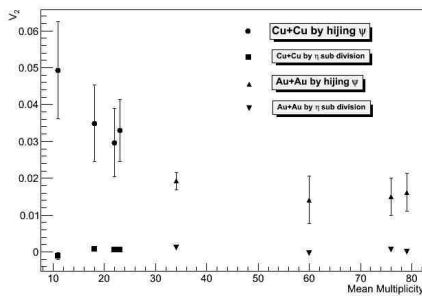
Fig. 2: Elliptic flow variation with mean multiplicity for \pi^+ at 200 GeV
