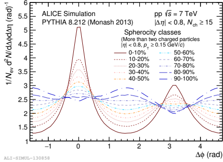
FIG. 1: Sphericity dependence of the leading-hadron azimuthal correlations for pp collisions at \sqrt{s} = 7 TeV.
