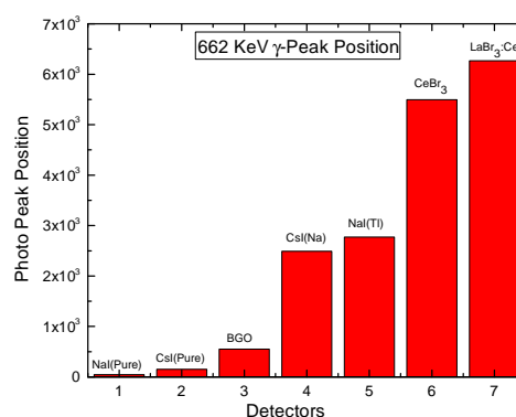
FIG. 1: 662 \gamma -ray Photo Peak Position from different scintillators.
