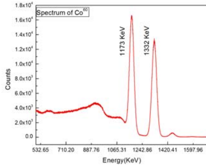
Fig.3: Energy spectrum using ^{60}\text{Co} source.
