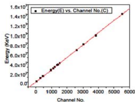
Fig.2: Energy calibration curve
