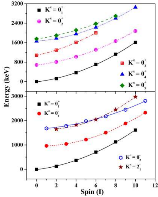
FIG. 1: The excitation energy vs spin has been plotted for the newly observed bands developed on the K^\pi = 0^- octupole band. See text for details.
