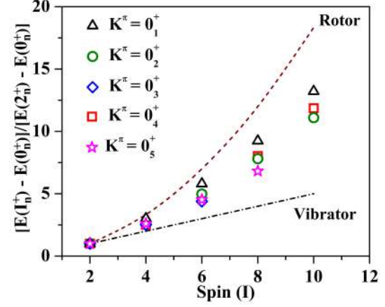
FIG. 2: The characteristic energy ratios are plotted as a function of spin for the excited 0^+ sequences proposed in the present work along with the known ones. See text for details.
