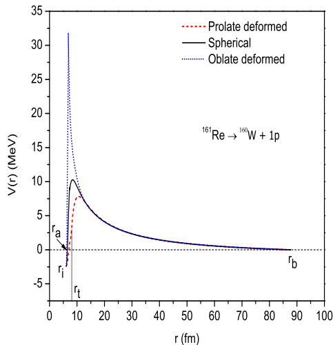
FIG. 1: Comparison of total potential V(r) of 1p emitting nucleus ^{161}\text{Re} , for spherical (solid line), prolate (dashed line) and oblate (dotted line) configurations.
