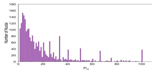
Fig. 3. Distribution of values of P_H
