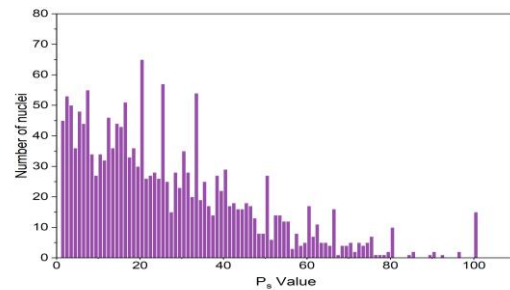
Fig. 1 Distribution of P_S values of all 1790 nuclei.
