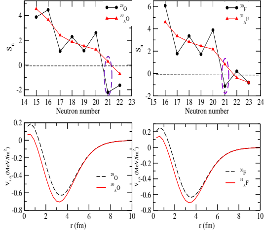
FIG. 1: One-neutron separation energy ( S_n ) for O and F isotopes and their hypernuclei. Spin-orbit interaction potential for ^{29}\text{O} , ^{30}\text{F} and ^{30}_{\Lambda}\text{O} , ^{31}_{\Lambda}\text{F} drip-line nuclei and the hypernuclei.
