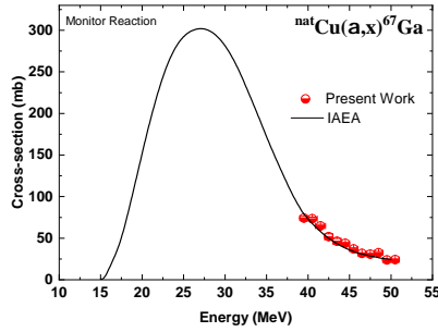
FIG. 2: Monitor reaction ^{nat}\text{Cu}(\alpha, x)^{67}\text{Ga} [1] overlap with IAEA recommended data [2] for the present experimental conditions.
