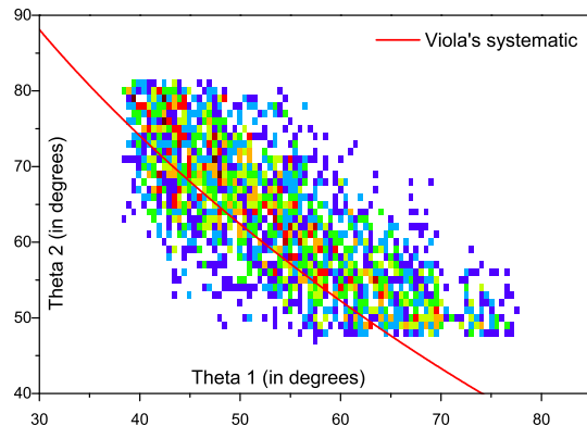
FIG. 3: The angular correlation between the fission fragments. The red line corresponds to angular correlation following Viola's systematic following full linear momentum transfer.
