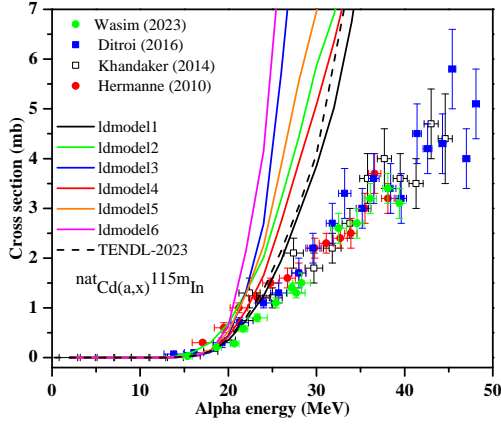
FIG. 2: Similar to Fig. 1, the theoretical calculation for CS of the ^{nat}\text{Cd}(\alpha,x)^{115m}\text{In} reaction compared with the experimental values reported by Wasim et al. [7], Ditroi et al. [9], Hermanne et al. [11] and Kandaker et al. [12] together with TENDL-2023 database [8].
