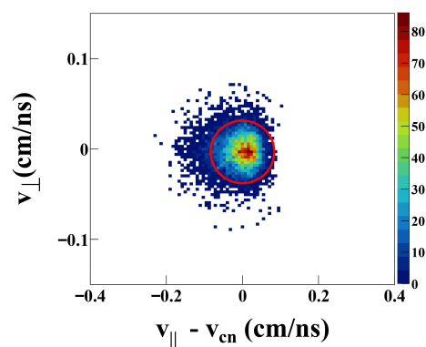
FIG. 1: Correlation between the two velocity components v_{\parallel} - v_{\text{cn}} vs v_{\perp} ( v_{\parallel} = parallel component and v_{\text{per}} = perpendicular component) of ^{30}\text{Si} + ^{160}\text{Gd} reaction at E_{\text{beam}} = 147.8 \text{ MeV} . The area inside the red contour represent FMT events used for mass and TKE distribution analysis.
