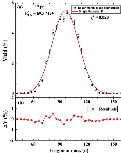
FIG. 2: (a) Mass distribution obtained for ^{190}\text{Pt}^* populated via ^{30}\text{Si} + ^{160}\text{Gd} reaction at E_{\text{beam}} = 147.8 MeV (black filled circles). FFMD fitted with single Gaussian along with the corresponding \chi^2 . (b) Residuals from the single Gaussian fitting showing the need to include an asymmetric fission mode around A_L \sim 80 .
