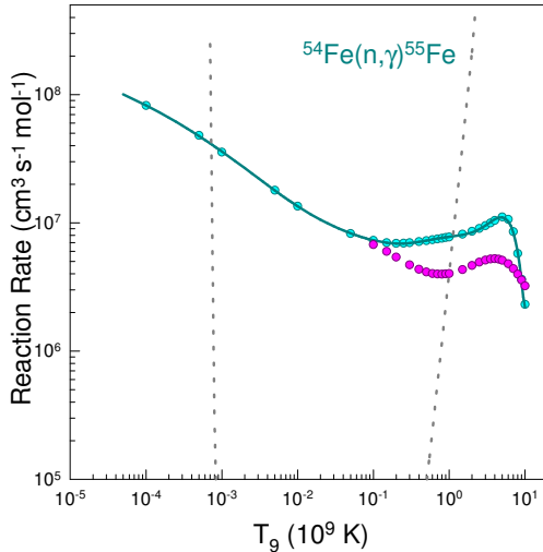
FIG. 1: The Hauser-Feshbach estimates of thermonuclear reaction rate per mole ( N_A \langle \sigma v \rangle ) for ^{54}\text{Fe}(n,\gamma)^{55}\text{Fe} versus temperature T_9 . The hollow circles (cyan) on the continuous line represent these estimates while the continuous line itself represents the polynomial fit. The solid circles (pink) represent the experimental data while the dotted line represents the JINA REACLIB reaction rate calculations [2, 3].
