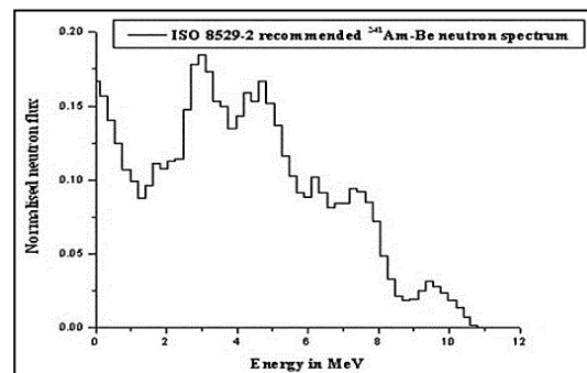
Fig. 2 ISO standard Am-Be neutron spectrum
